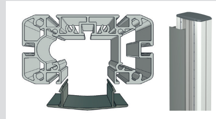
Close-up: support extrusions center column cable channel
